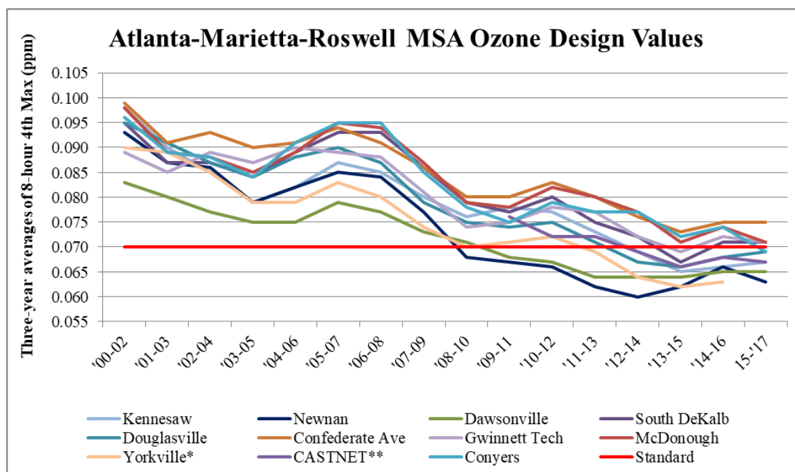
Figure 2: Atlanta-Marietta-Roswell MSA Ozone Design Values, 2000-2017
