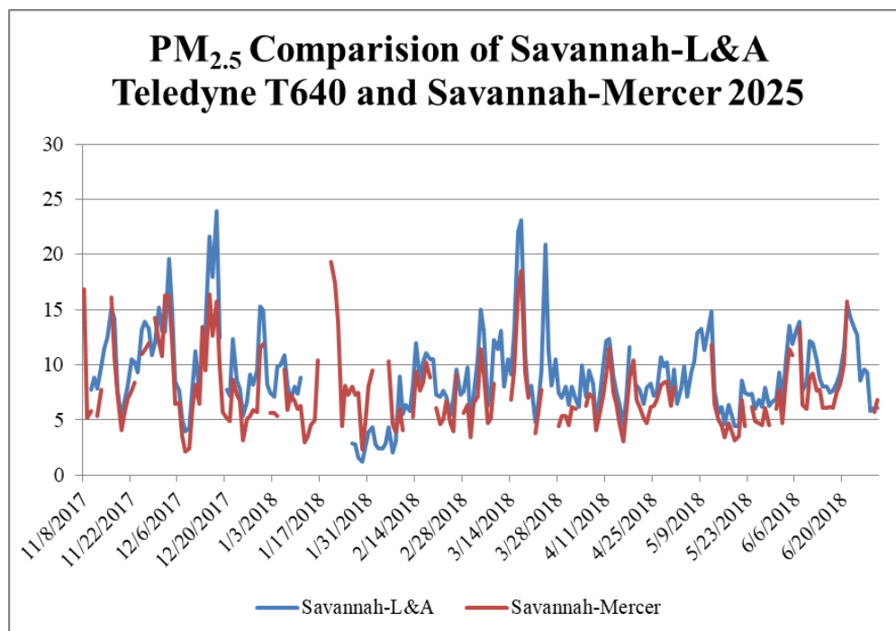
Figure 3: Comparison of PM 2.5 Data
